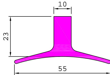
18570 0.942 kg/m
