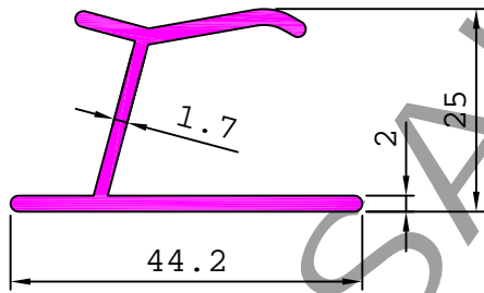
18577 0.351 kg/m
