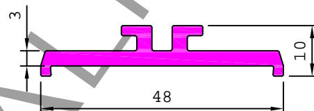
S4091 0.517 kg/m
