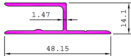
S4104 0.827 kg/m
